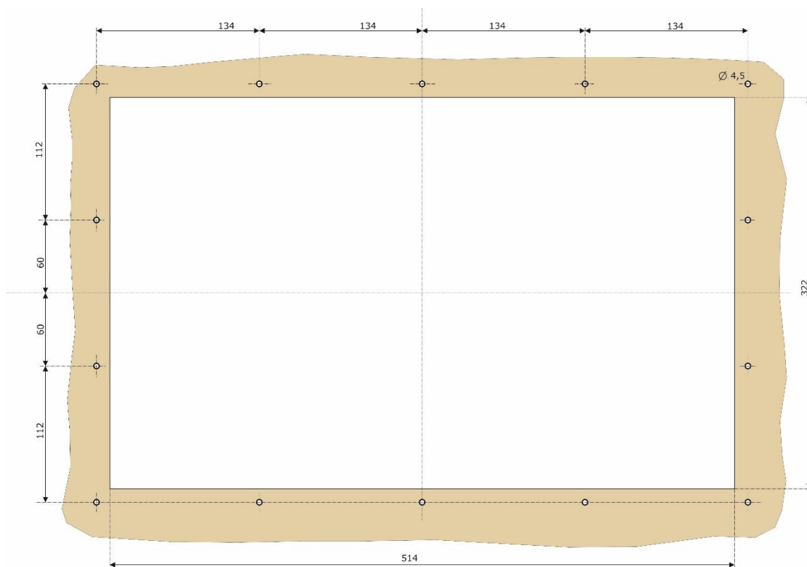
Cutout for Operator Panel with 240 keys; 514 x 322 mm 2
